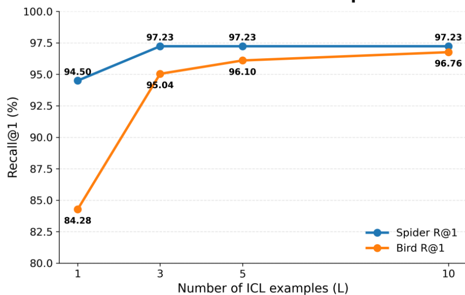
Effect of More ICL Examples
