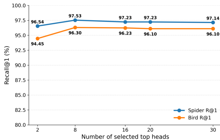
Effect of Selected Heads
